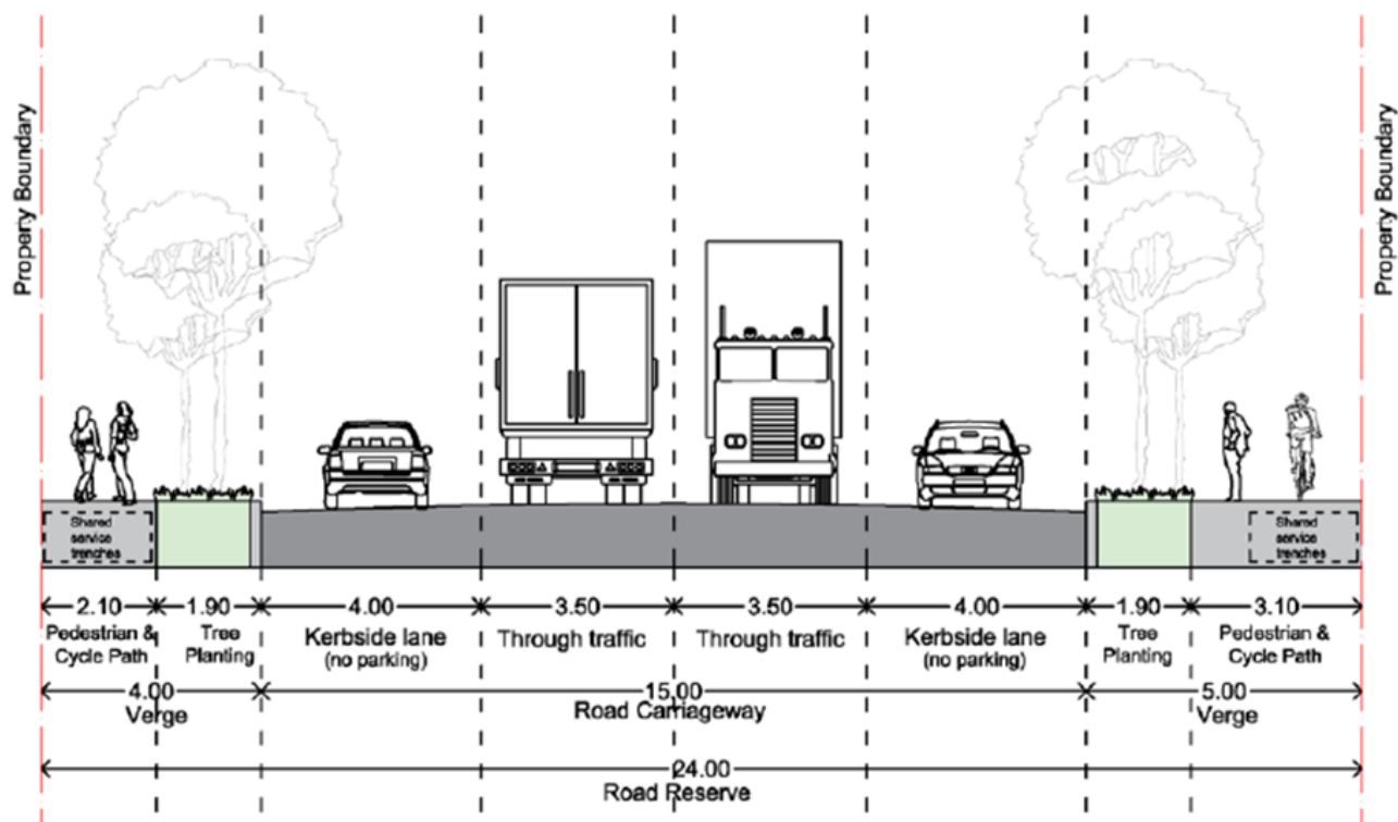
Figure E18.8 Collector Road Cross Section
